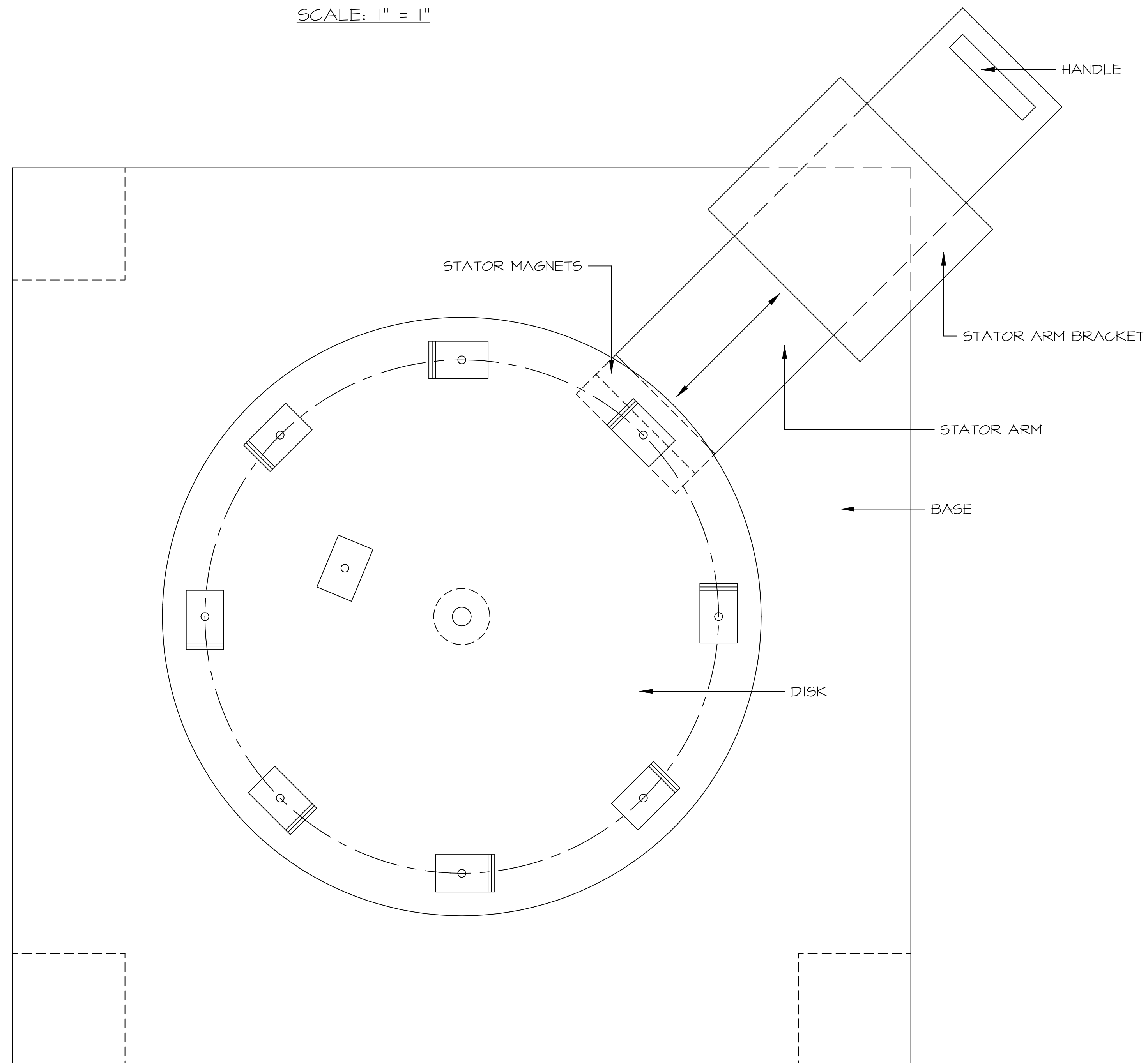
MOTOR ASSEMBLY - FRONT VIEW
