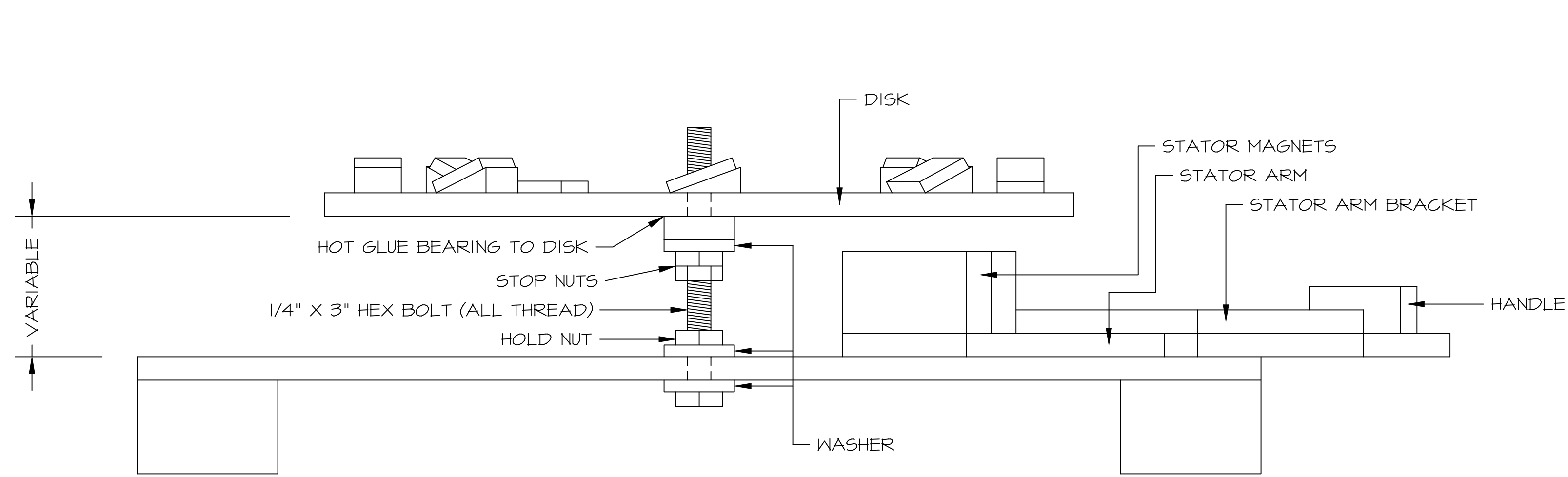
MOTOR ASSEMBLY - FRONT VIEW
