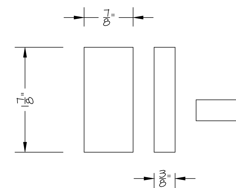
LG. CERAMIC MAGNETS (STOCK - 2 EA.)
