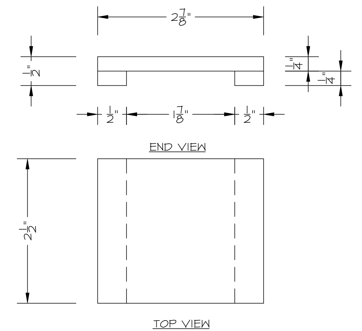
STATOR ARM BRACKET (1 EA.)
