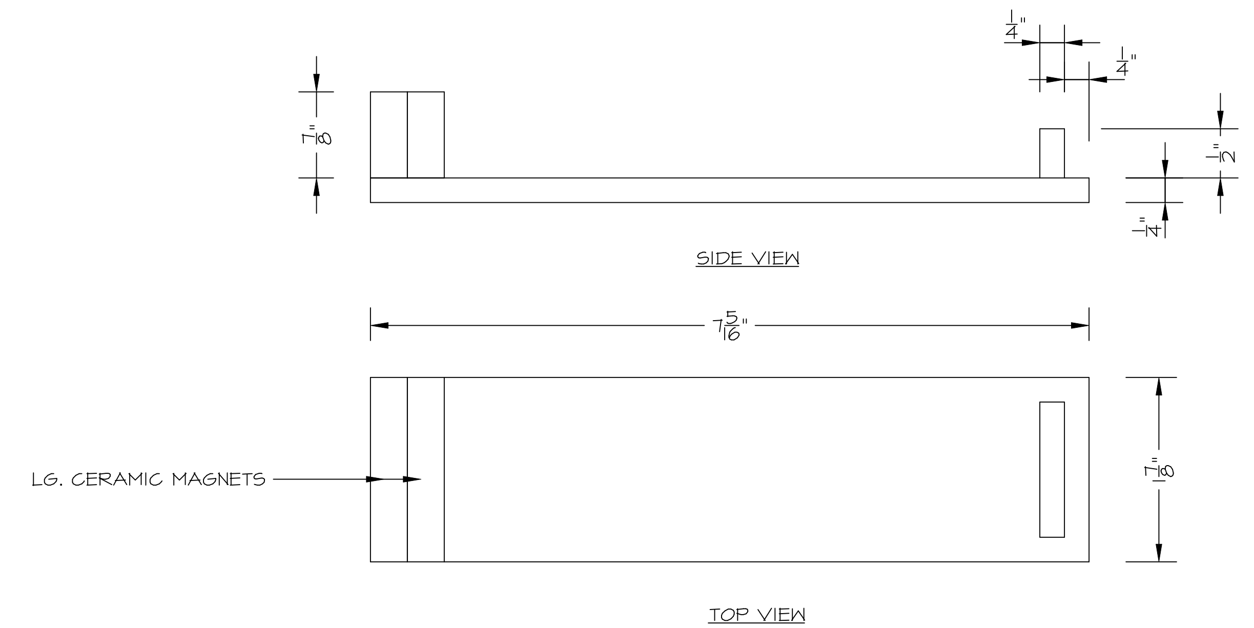
STATOR ARM (1 EA.)
