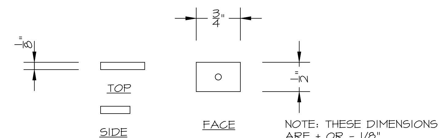
SM. CERAMIC MAGNETS (STOCK - 9 EA.)
